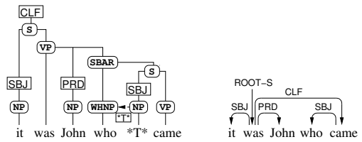
Figure 5: A cleft sentence and its dependency representation.
