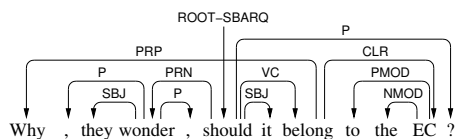
Figure 3: Dependency tree by the new procedure.
